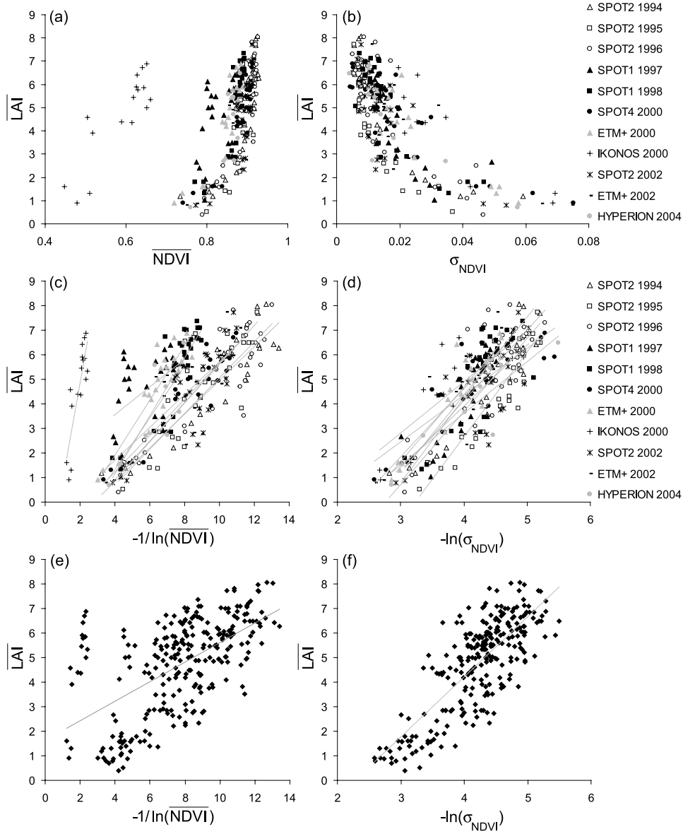
Figure 4. Comparison of (a) \overline{\text{LAI}}-\text{NDVI} and (b) \overline{\text{LAI}}-\sigma_{\text{NDVI}} for 11 satellites. \overline{\text{LAI}} as a function of (c) -1/\ln(\text{NDVI}) and (d) -\ln(\sigma_{\text{NDVI}}) (see equations (1) and (2) in text). Gray lines are linear regressions ( r^2 are given in Table 3). (e, f) Same as Figures 4c and 4d but with all 259 points together.
