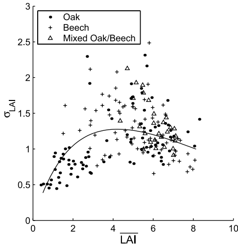
Figure 3. Standard deviation of the LAI ( \sigma_{\text{LAI}} , \text{m}^2/\text{m}^2 ) as a function of the mean stand LAI ( \overline{\text{LAI}} , \text{m}^2/\text{m}^2 ). Stand LAIs are obtained from ground measurements (40 to 150 PCA LAI-2000 samples per stand). Plots are presented by species. All 197 forest-stand samples between 1994 and 2004 are presented in this graph. Solid line represents the results given by the Weibull model (see Appendix A).
