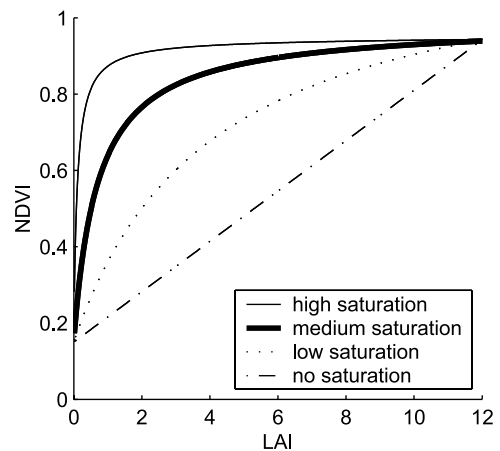
Figure 1. Four LAI-NDVI relationships created to test the theoretical basis of the \overline{\text{LAI}}\text{-}\sigma_{\text{NDVI}} relationship using modeling. They go from a highly saturated one to a linear one.
