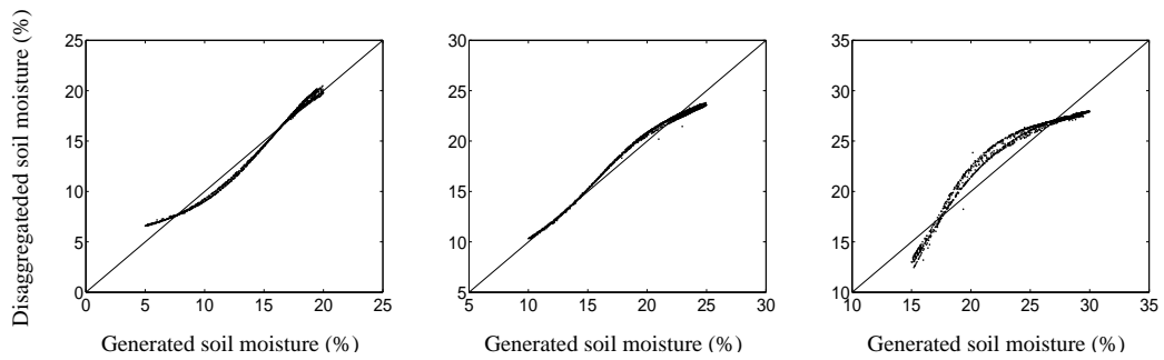
Fig. 6. Soil moisture disaggregated by the method as a function of the generated soil moisture. Three ranges of soil moisture are considered: 5–20 %, 10–25 % and 15–30 %.
