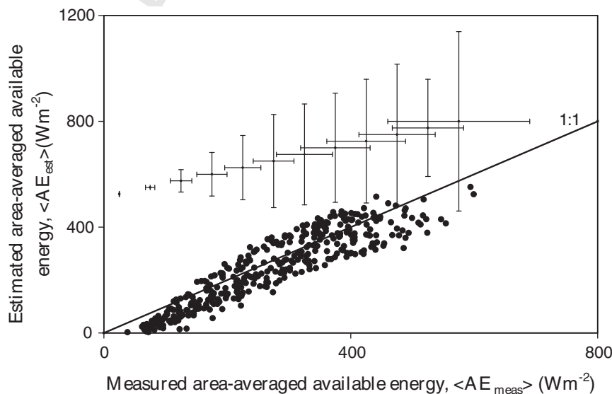
Fig. 6. Comparison between the estimated— \langle AE_{est} \rangle , obtained using the aggregation approach—and measured— \langle AE_{meas} \rangle , obtained as area weighted averages of those measured over the three sites—area-averaged available energy during the study period (DOYs 204–225). The error bars represent the average uncertainty of the fluxes for each 50 \text{ W m}^{-2} interval.
