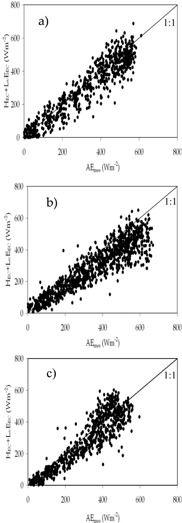
Figure 4. Comparison between measured available energy ( AE=R_n - G ) and the sum of eddy covariance measurements ( H_{EC} + L_v E_{EC} ) over the three sites (4a for Agdal, 4b for R3 and 4c for Sâada).
