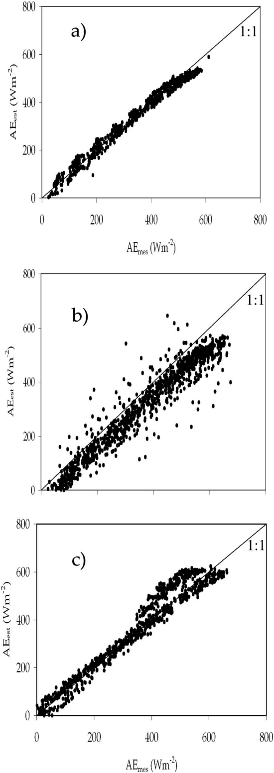
Figure 8. Comparison between estimated ( AE_{est} ) and measured ( AE_{mes} ) available energy over the three sites Agdal (a), R3 (b), and Sâada (c).
