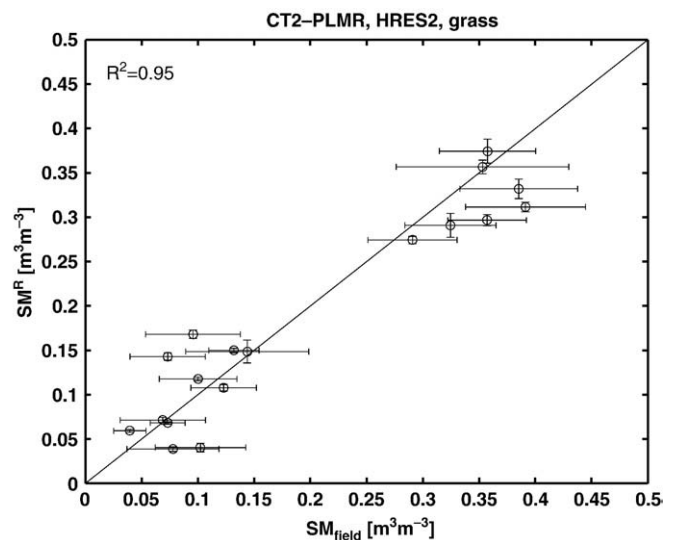
Fig. 5. Soil moisture retrievals from CT2-PLMR flights over grass in the HRES2 area based on a 2-P inversion ( SM^R , \tau_{NAD} ) with the roughness fit in Eq. (6). Bars indicate the standard deviation of the measured field soil moisture ( SM_{field} ) and the retrieved soil moisture ( SM^R ).
