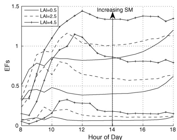
Fig. 9. Mean diurnal cycle of modeled soil evaporative fraction, from 4 January 2003 to 21 May 2003, for constant surface soil moisture values of 0.1, 0.2 and 0.3 m 3 m -3 , and constant LAI values of 0.5, 2.5 and 4.5.
