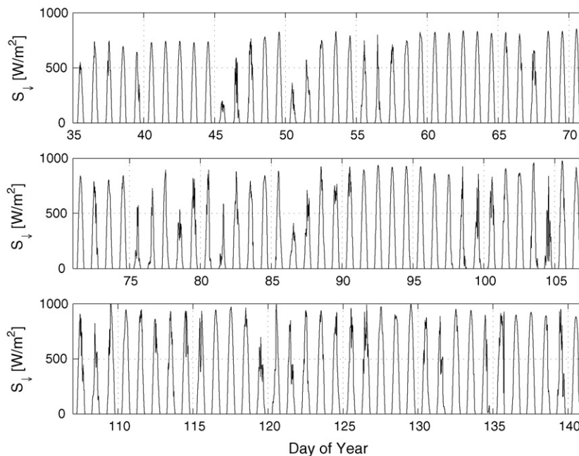
Fig. 4. Observed solar incoming shortwave radiation in \text{W m}^{-2} over R3-B123 field in 2003.
