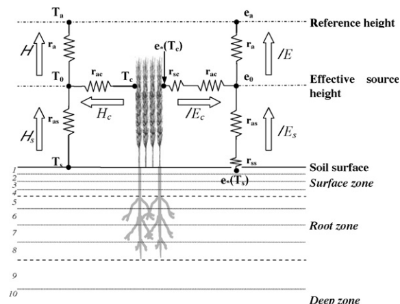
Fig. 1. Dual source (soil-canopy) resistance network. This model is coupled with a 10-layer diffusive soil model for heat and moisture transfer.
