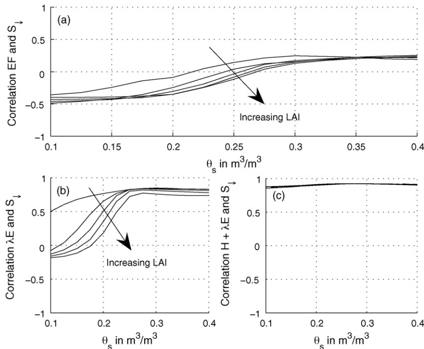
Fig. 12. Cross-correlation between (a) EF, (b) LE, (c) H + \lambda E and solar incoming radiation over the 4 January–21 May 2003 modeling period for constant LAI values of 0.5, 1.5, 2.5, 3.5 and 4.5.
