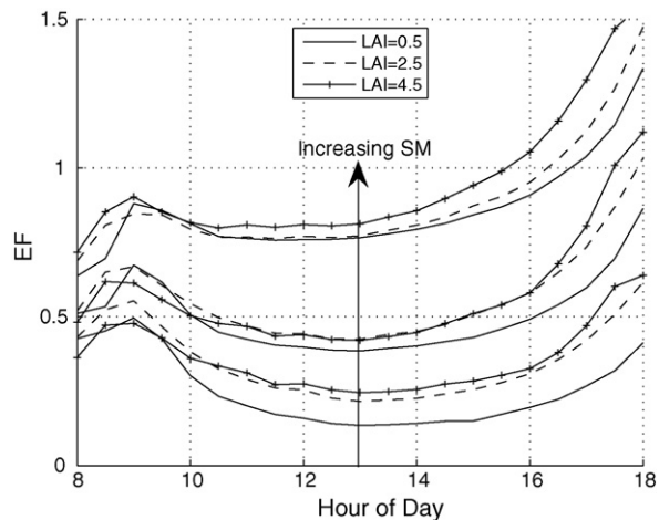
Fig. 8. Mean diurnal cycle of modeled evaporative fraction, from 4 January 2003 to 21 May 2003, for constant surface soil moisture values of 0.1, 0.2 and 0.3 m 3 m -3 , and constant LAI values of 0.5, 2.5 and 4.5.
