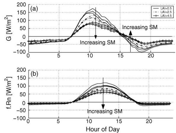
Fig. 6. Mean daily cycle of the SVAT modeled soil heat flux (a) and soil heat flux taken as fraction of the net radiation (b); for soil surface moisture values of 0.1, 0.2, 0.3 \text{m}^3 \text{m}^{-3} .
