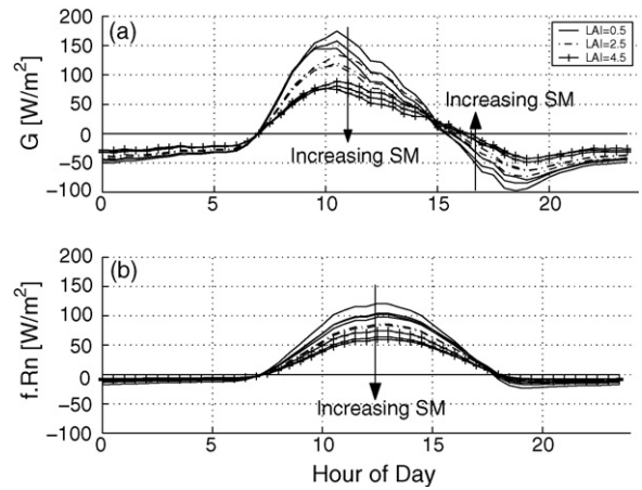
Fig. 6. Mean daily cycle of the SVAT modeled soil heat flux (a) and soil heat flux taken as fraction of the net radiation (b); for soil surface moisture values of 0.1, 0.2, 0.3 \text{m}^3 \text{m}^{-3} .
