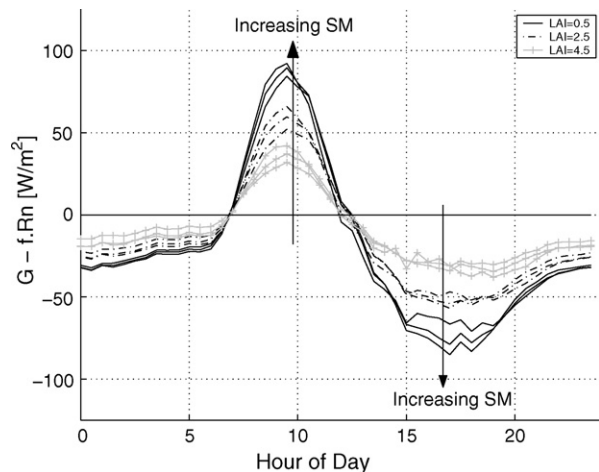
Fig. 7. Mean daily cycle of the difference between the SVAT modeled soil heat flux and the net radiation proportional heat flux; for soil surface moisture values of 0.1, 0.2, 0.3 \text{m}^3 \text{m}^{-3} .
