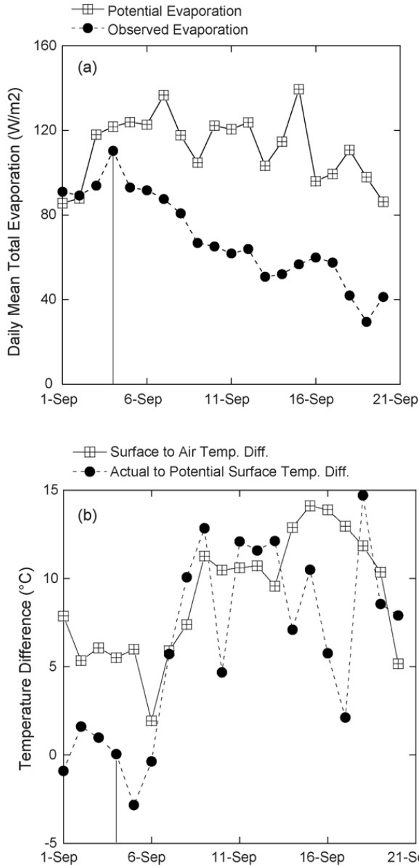
Fig. 3. Same as Fig. 1 in the case of the SALSA grassland site at maximum development.
