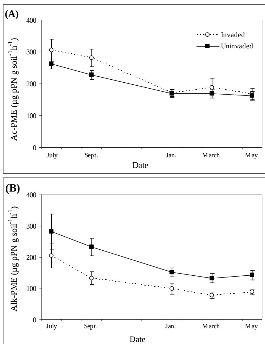
Figure 3: Seasonal variation of soil phosphomonoesterase (PME) activity in plots invaded by early Goldenrod and adjacent, uninvaded plots. (A) Ac-PME, (B) Alk-PME. Means (n=6) and standard deviations.
