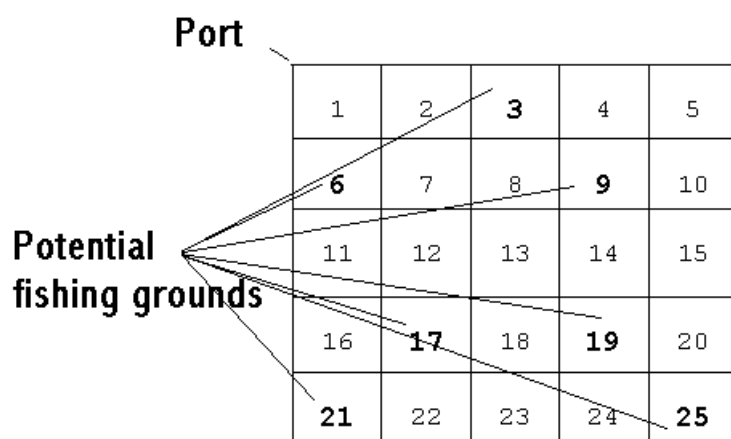
Fig. 1. Simulated world.
