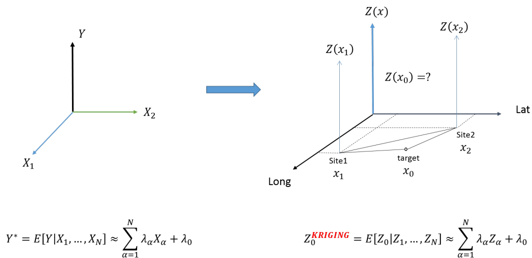
Figure 15: Regression: estimating the parameters of the regression to best explain Y by a linear combination of X_1 and X_2 . Kriging: choosing the parameters of the linear combination of Z(x_1) and Z(x_2) that allows a BLUE estimation of Z(x_0)
