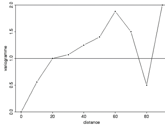
Figure 3: Empirical variogram.
